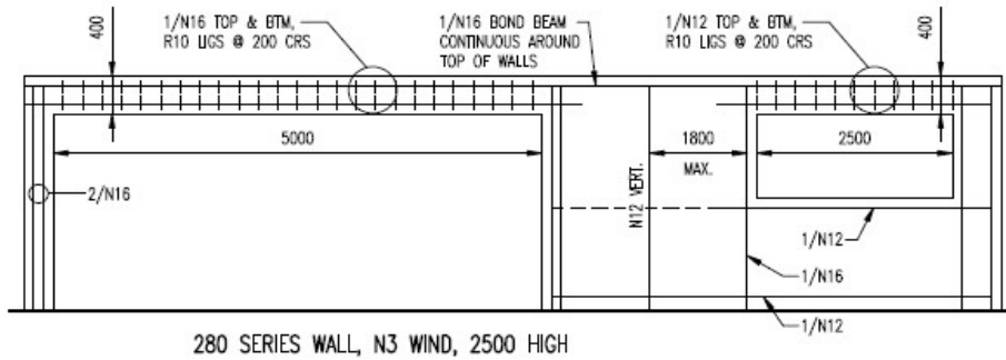
Fig 2i: 2500 High Wall, N3 Wind Rating, 280 Series ECO-Block (Max. roof load width: 6.8m)
