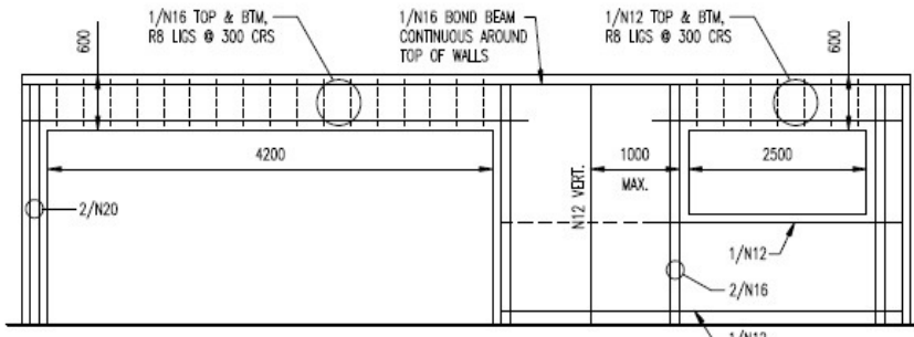
230 SERIES WALL, N4/C1 WIND, 2700 HIGH
