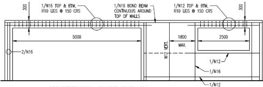
280 SERIES WALL, N2 WIND, 2400 HIGH
