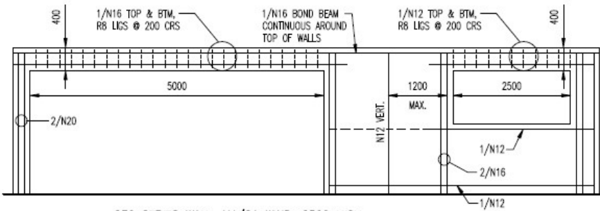
230 SERIES WALL, N4/C1 WIND, 2500 HIGH
